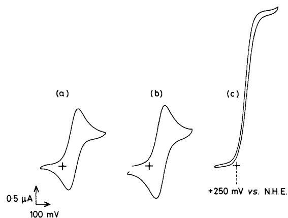
Figure 2. D.c. cyclic voltammograms ( 5 \text{ mV s}^{-1} ) recorded at a 4 mm diameter gold disc working electrode. (a) 0.25 mM ferroceneboronic acid in 50 mM Tris-HCl, 10 mM KCl, pH 7.6; (b), as (a), with the addition of o -cresol and p -cresol methylhydroxylase to final concentrations of 7 mM and 0.53 \mu\text{M} , respectively. (c), as (a), with the addition of p -cresol and p -cresol methylhydroxylase to final concentrations of 7 mM and 0.53 \mu\text{M} , respectively.
